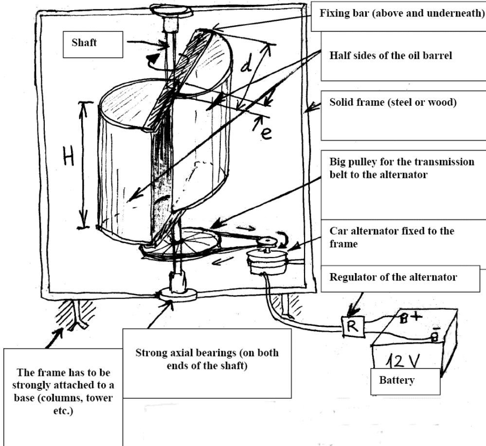
Fig. 3.1-1 Principle of a ECODRUM REGEN SYSTEM
