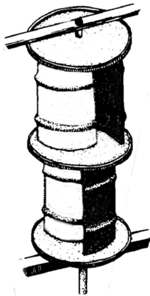
Fig. 3.2-1 Two-barrel-ECODRUM REGEN SYSTEM = double power, double torque, same rotation speed
