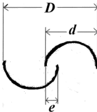
Fig. 3.1-2 Definition of the values D , d and e
